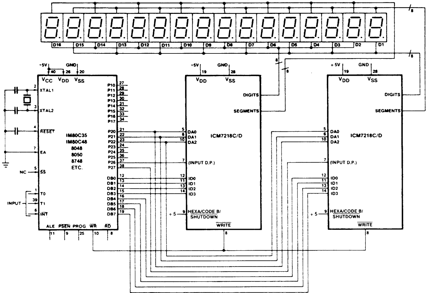
FIGURE 11. 16-DIGIT DISPLAY
