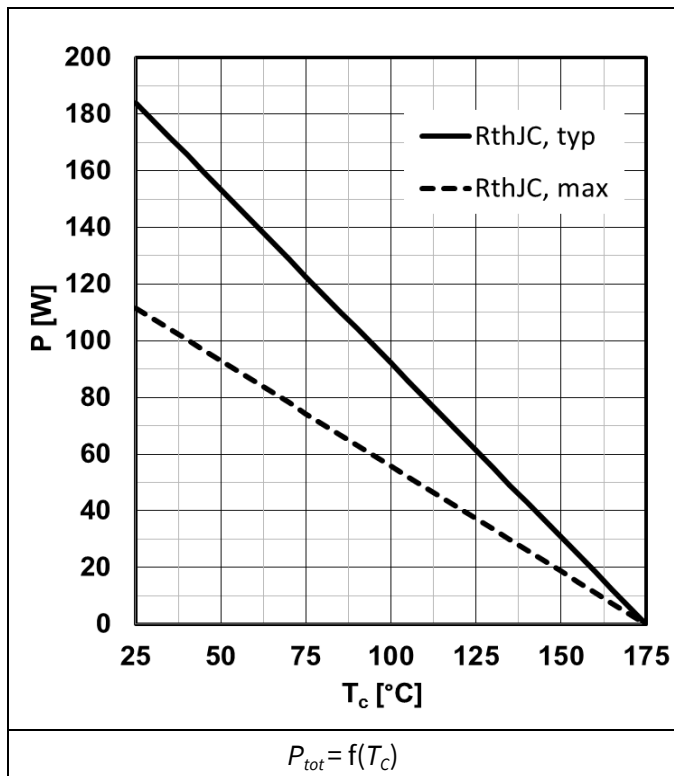
Figure 1 Power dissipation
