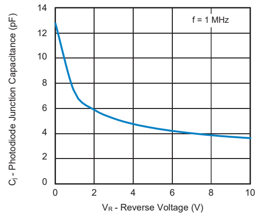
Fig. 10 - Photodiode Junction Capacitance vs. Reverse Voltage
