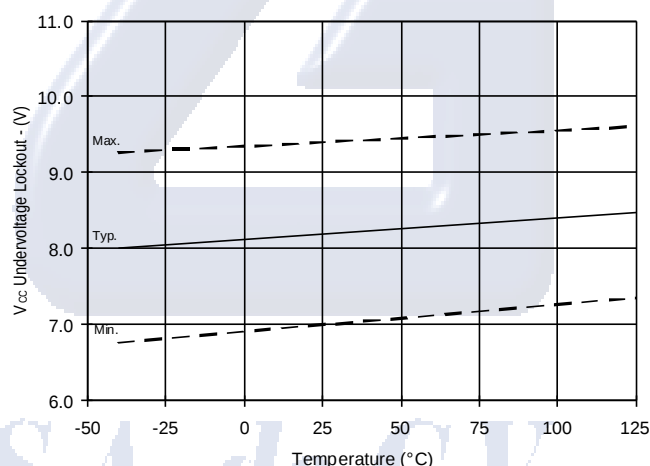
Figure 25. V_{CC} Undervoltage (-) vs. Temperature
