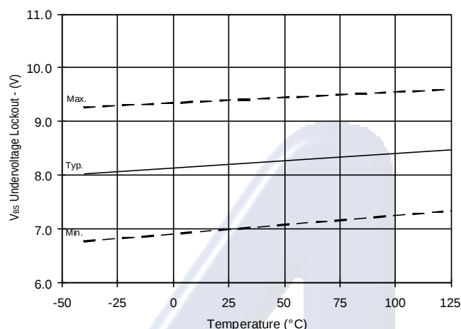
Figure 23. V_{BS} Undervoltage (-) vs. Temperature
