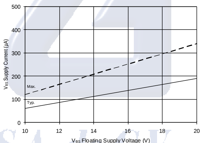
Figure 17B. V BS Supply Current vs. Voltage
