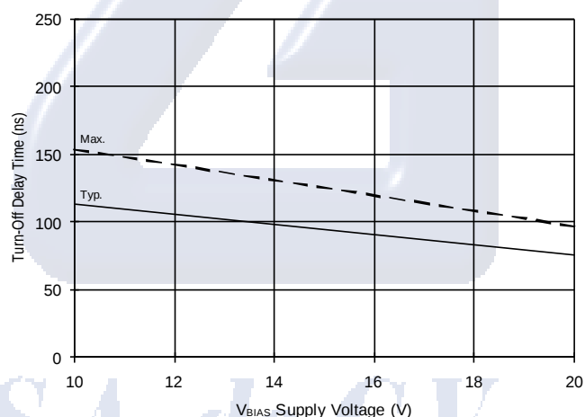
Figure 8B. Turn-Off Time vs. Voltage
