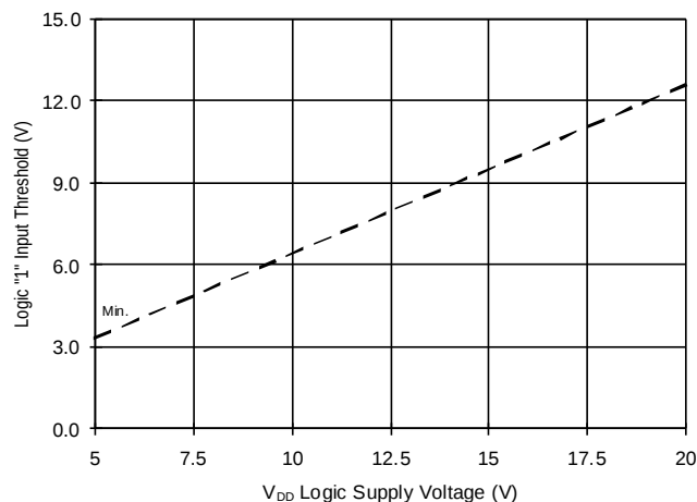
Figure 12B. Logic "1" Input Threshold vs. Voltage
