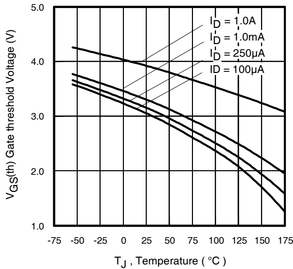
Fig. 16. Threshold Voltage V_{GS(th)} Vs. Temperature
