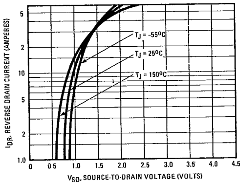
Fig. 7 – Typical Source-Drain Diode Forward Voltage
