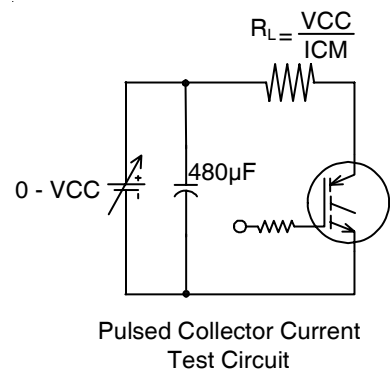
Figure 20. Pulsed Collector Current Test Circuit
