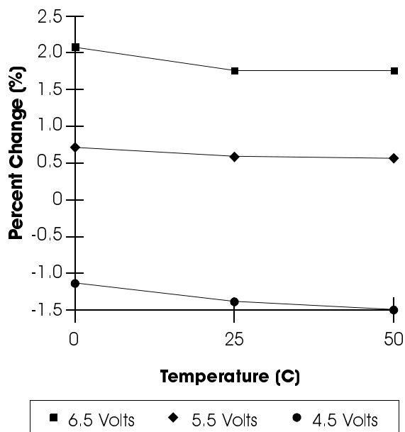
Chart 8: Oscillator Stability
