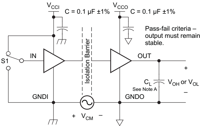
Figure 17. Common-Mode Transient Immunity Test Circuit
