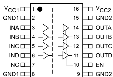
DW Package 16-Pin SOIC ISO7340x Top View
