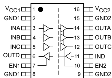
DW Package 16-Pin SOIC ISO7341x Top View
