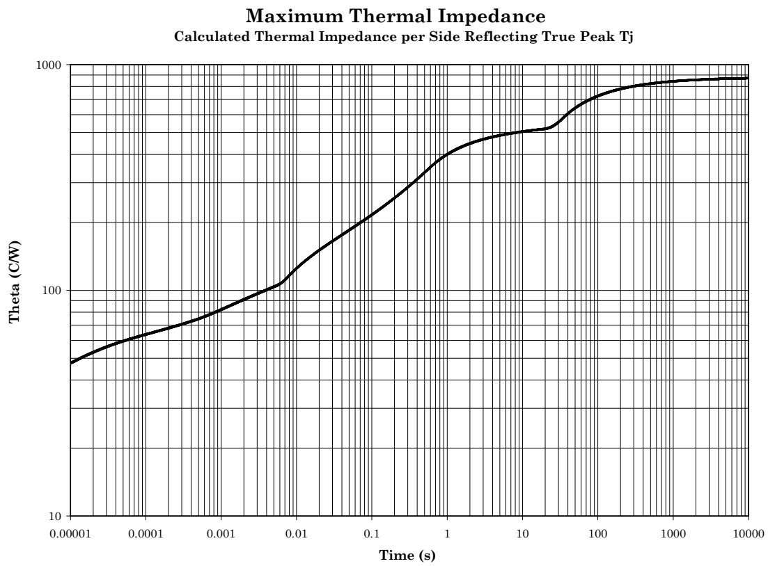
FIGURE 5. For each side: Thermal resistance (RHA) = 875°C/W, P_t = 200 mW.
