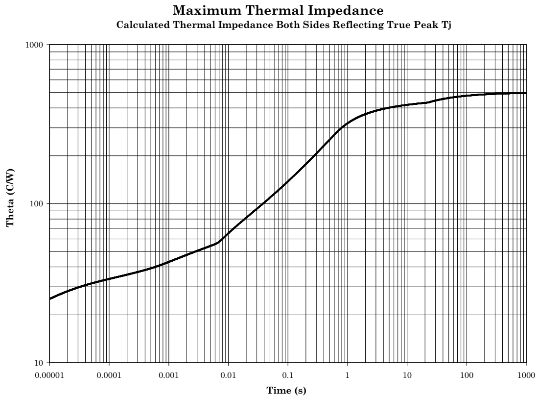
FIGURE 6. Both sides: Thermal resistance (RHA) = 500°C/W, Pt = 350 mW.
