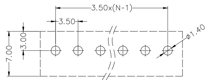
Recommended P.C.B Layout(Top Side)
