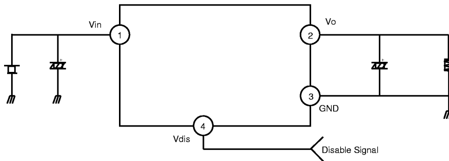
FIG.1 APPLICATION CIRCUIT
