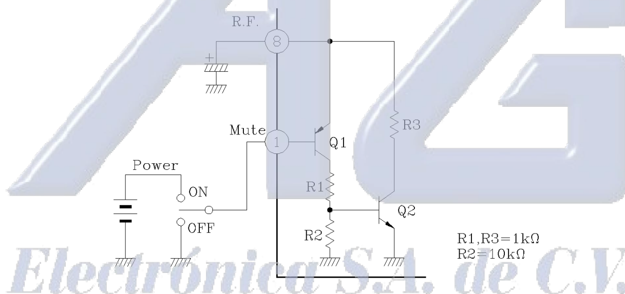
Fig.4 Mute Circuit
