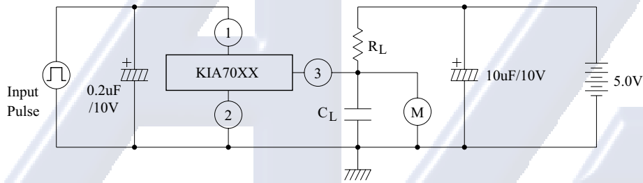
APPLICATION CIRCUIT
