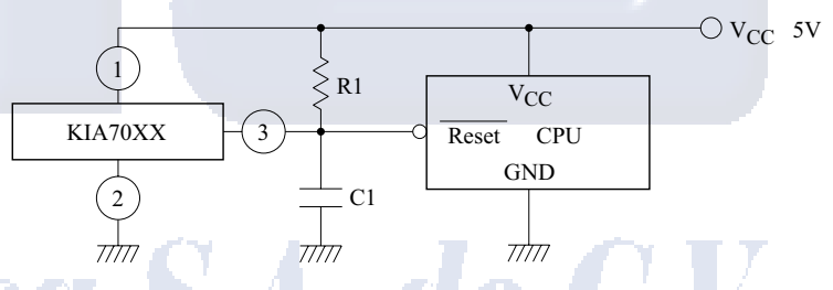
(2) CPU RESETTING
