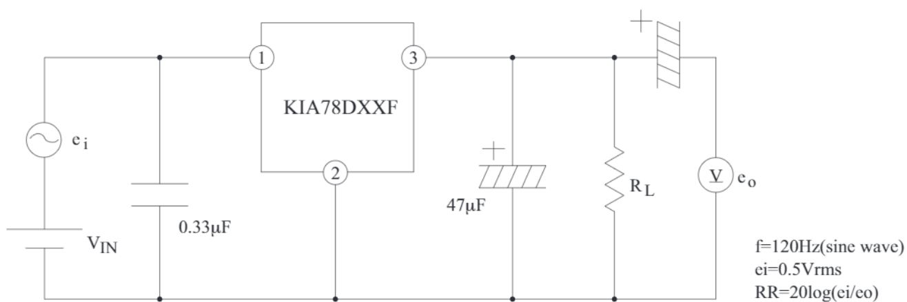
Fig. 1-2 Ripple Rejection Test Circuit
