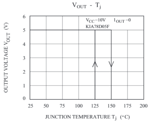
Fig 4. Thermal Cutoff Circuit Characteristics.
