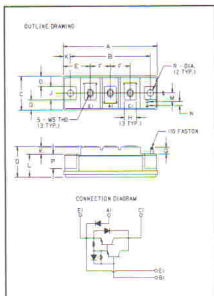
600 Volt KR224505 Outline Drawing
