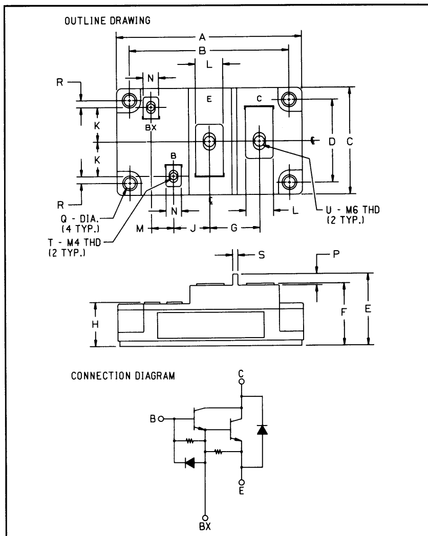
Outline Drawing
