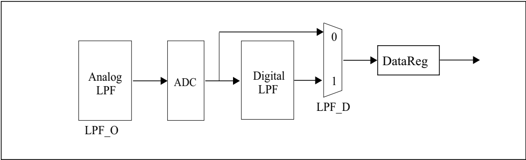
Figure 9. LPF chain block diagram
