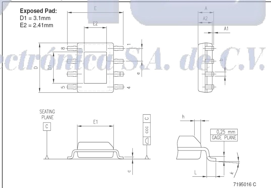
Figure 20. Package dimensions
