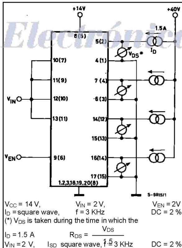
Figure 5 : R_{DS} \text{ (on)} .
