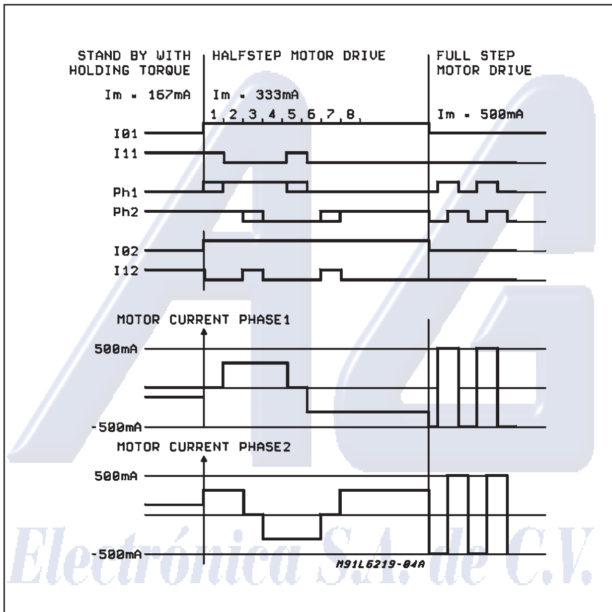
Figure 3: Principle Operating Sequence
