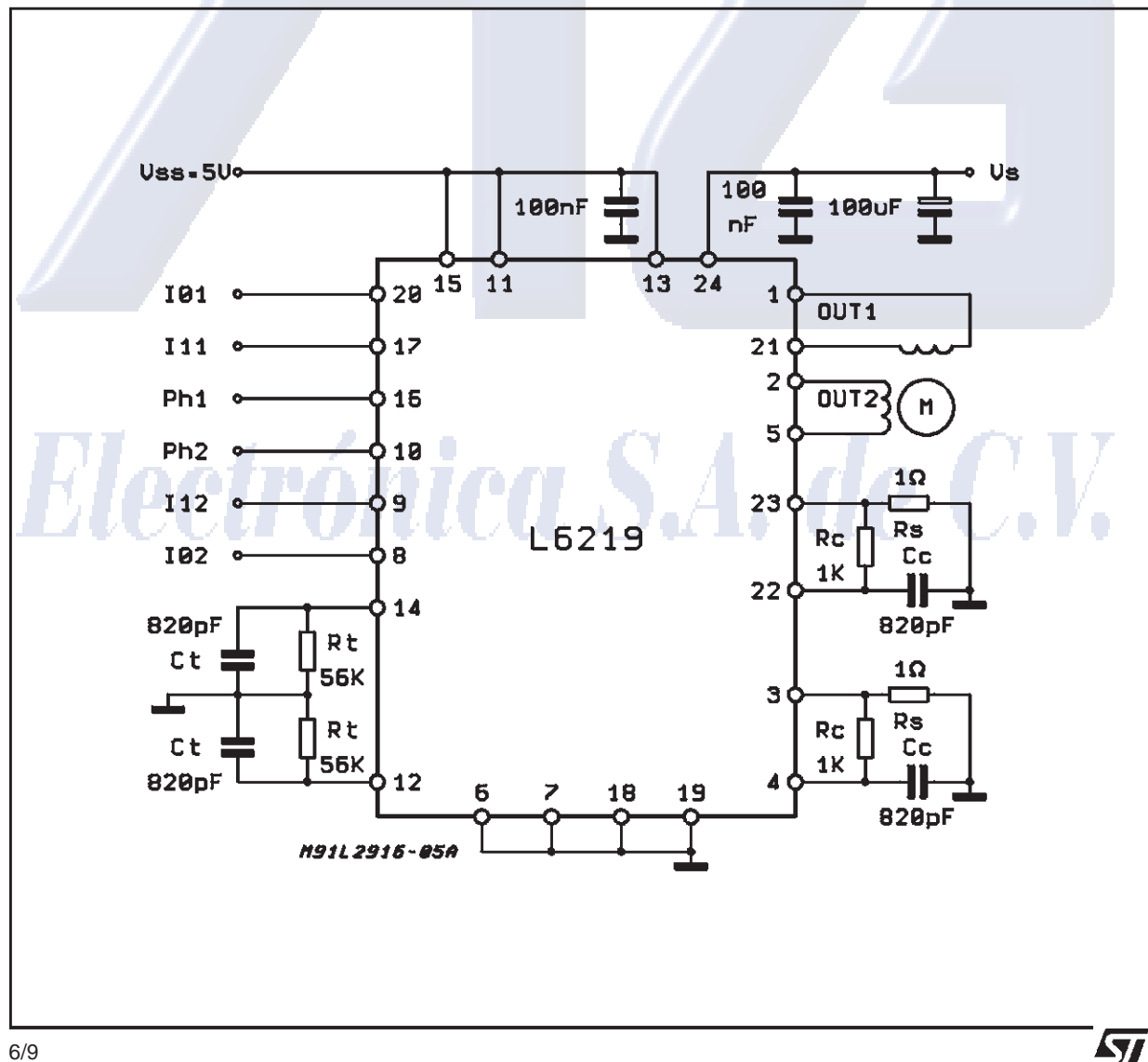
Figure 4: Typical Application Circuit. (Pin out referred to DIP24 package)
