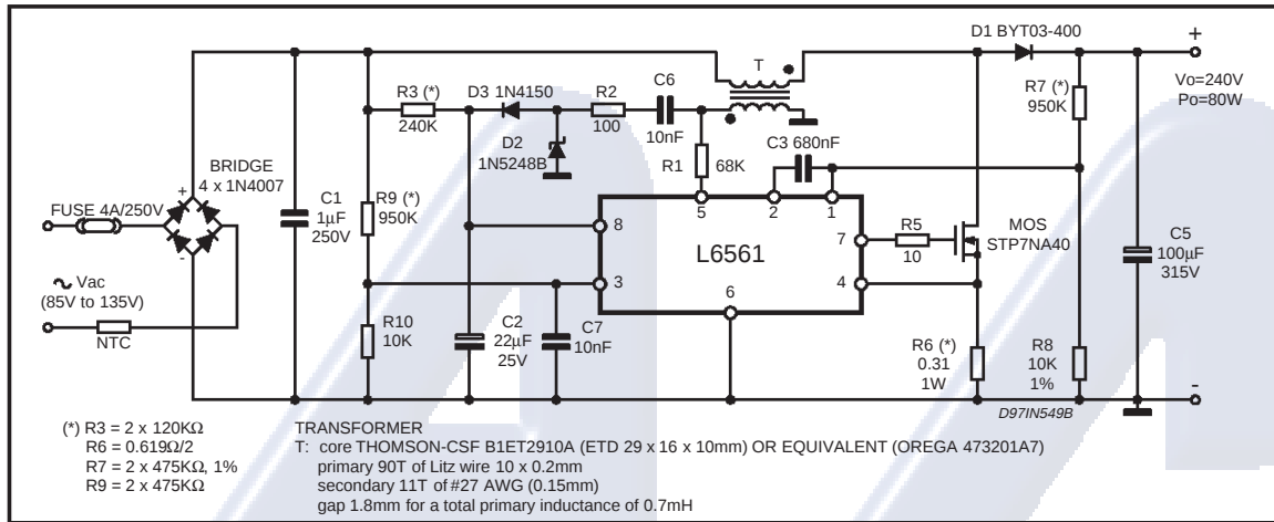
Figure 4. Typical Application Circuit (120W, 220VAC)
