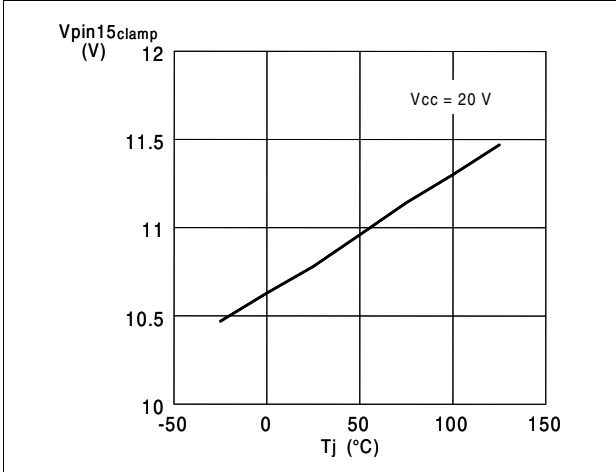
Figure 31. Gate-drive clamp vs T_J
