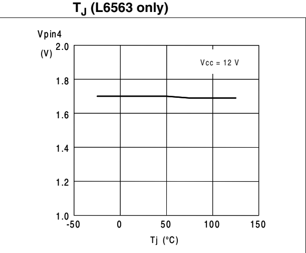
Figure 14. Ic latch-off level on current sense vs T_J (L6563 only)
