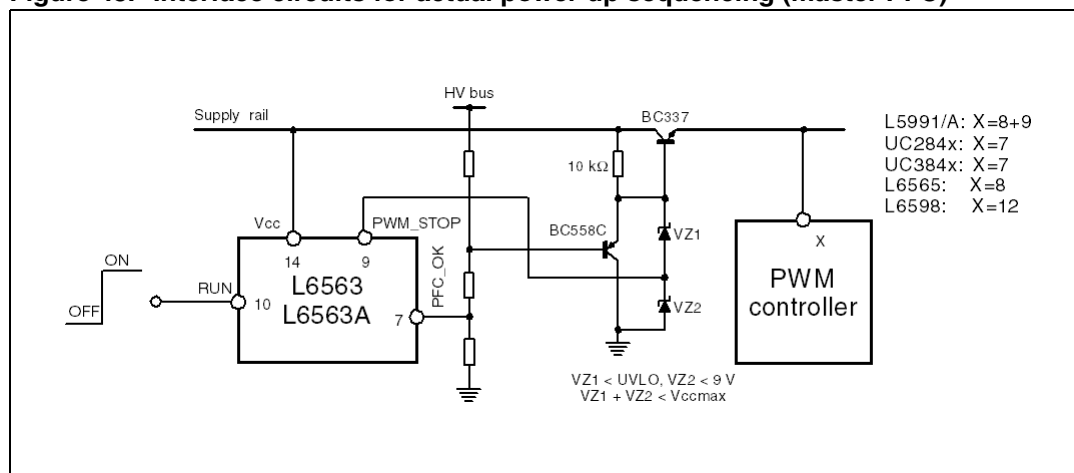
Figure 43. Interface circuits for actual power-up sequencing (master PFC)
