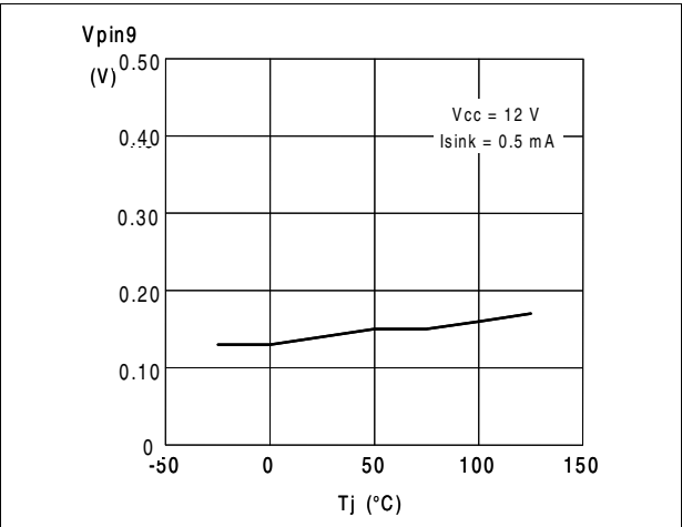
Figure 26. PWM_STOP low saturation vs T_J
