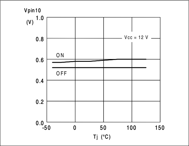
Figure 24. PWM_LATCH high saturation vs T_J
