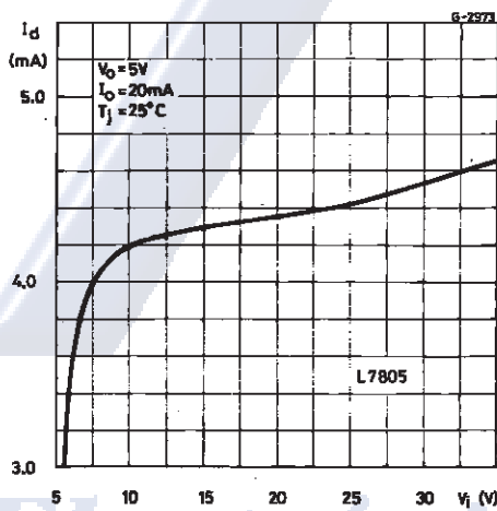
Figure 13 : Fixed Output Regulator.
