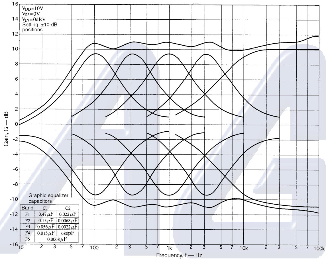
f_0 (Center Frequency) Characteristics
