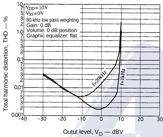
THD – Output Level Characteristics (1)
