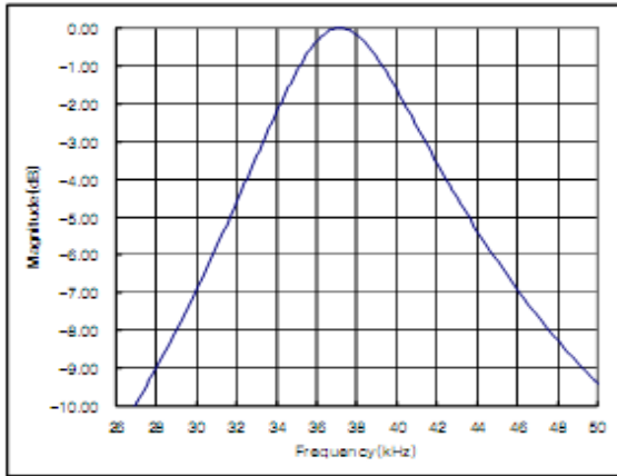
Figure 2. Typical Band-pass Curve
