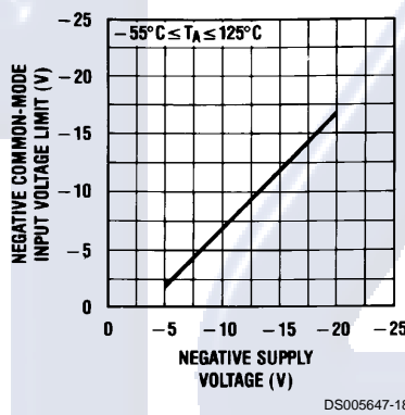
Negative Common-Mode Input Voltage Limit
