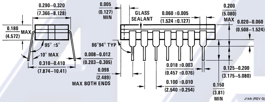
Ceramic Dual-In-Line Package (J) Order Number LF147J, LM147J-SMD or LF147J/883 NS Package Number J14A
