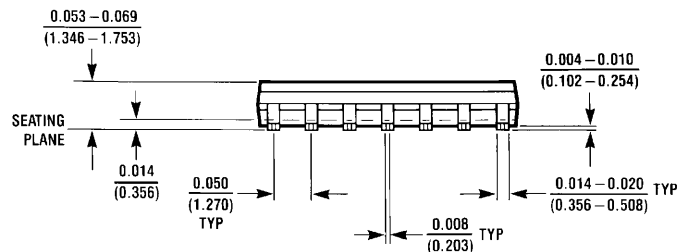
S.O. Package (M) Order Number LF347M or LF347MX NS Package Number M14A
