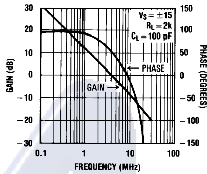
Bode Plot
