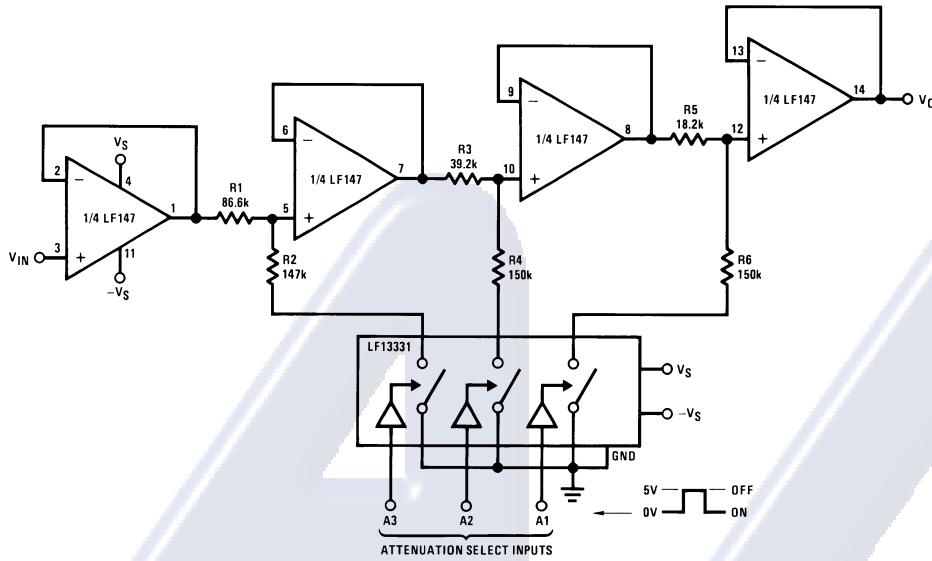
Digitally Selectable Precision Attenuator
