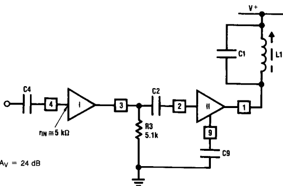
FIGURE 9. Receiver Section
