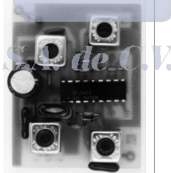
FIGURE 7. PCB Layout, Stuffing Diagram and Complete RX Module for Typical Application Circuit of Figure 5
