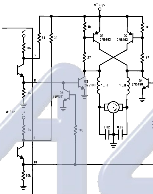
FIGURE 16. Digital Bridge Motor Drive
