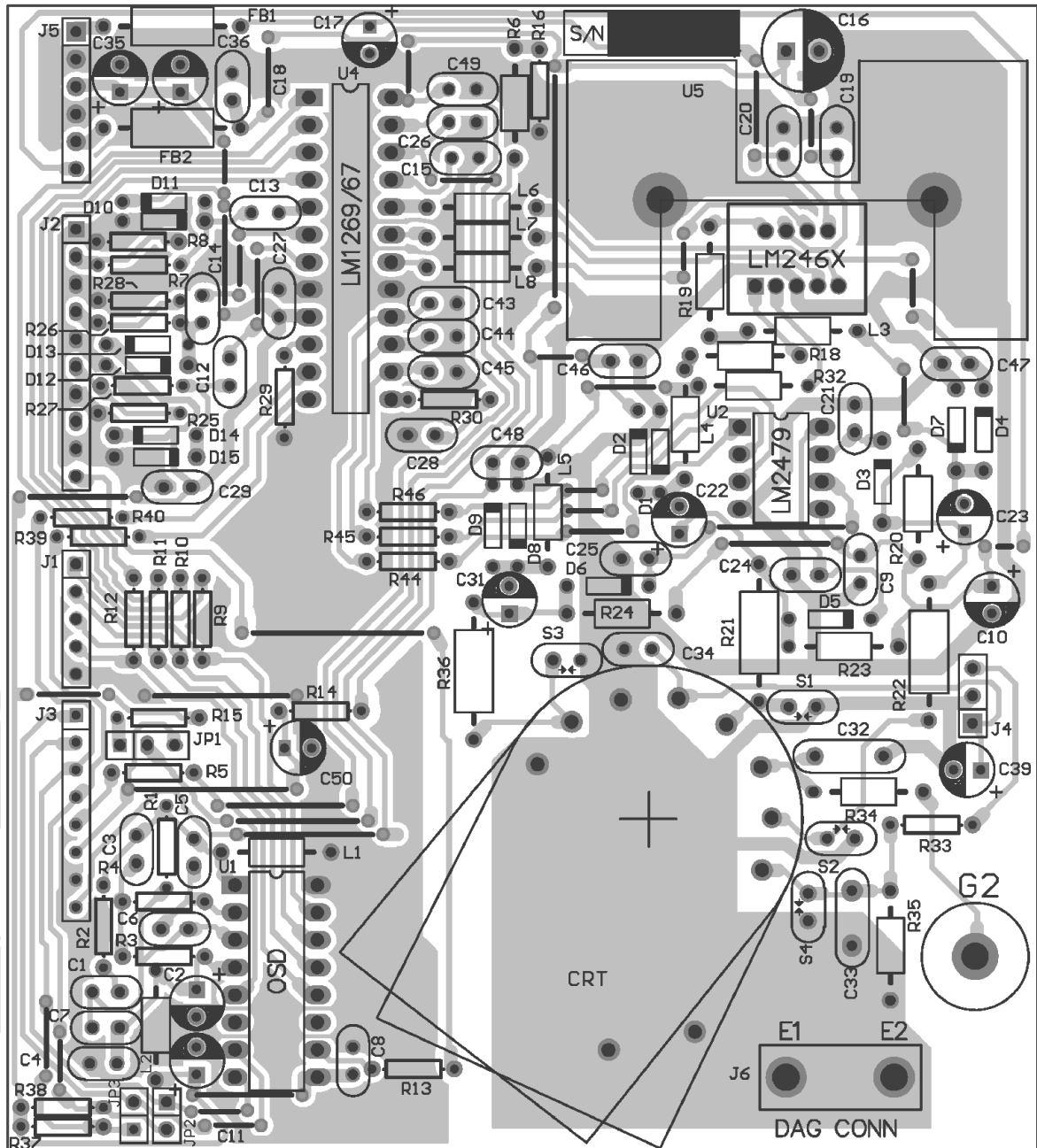
FIGURE 7. NSC LM26X/246X Demo Board Layout
