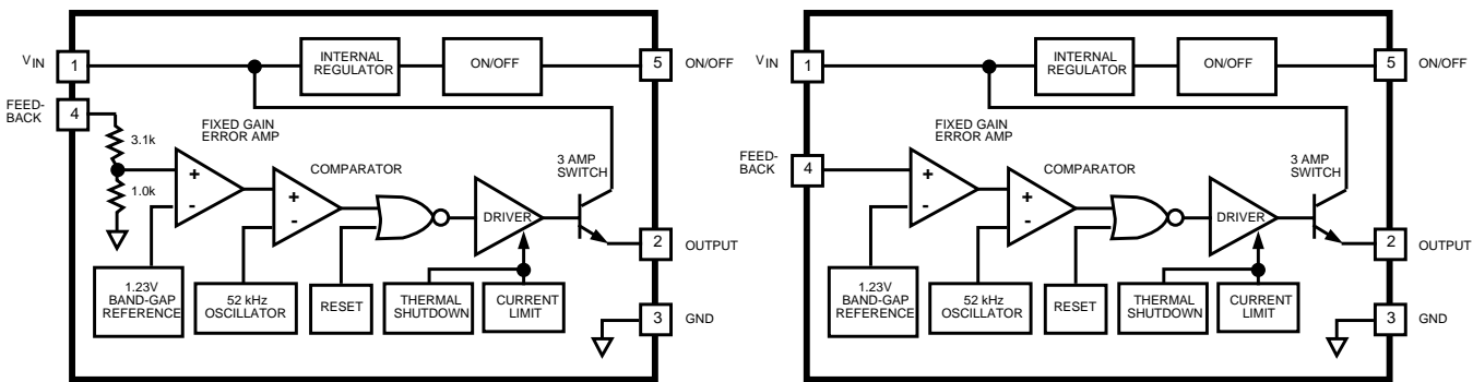
Fixed Regulator
