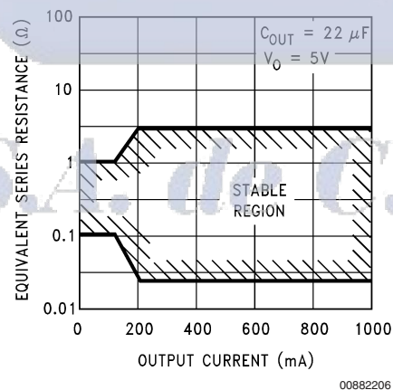
FIGURE 1. ESR Limits
