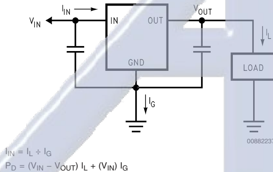
FIGURE 2. Power Dissipation Diagram
