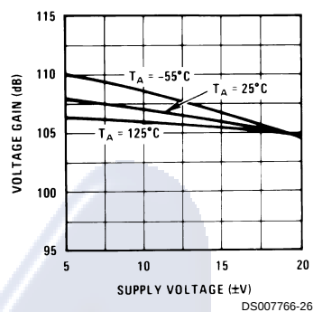
Voltage Gain
