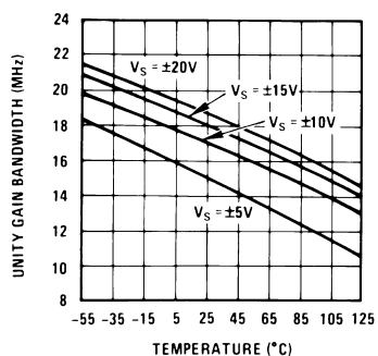
Unity Gain Bandwidth
