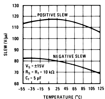
Voltage Follower Slew Rate
