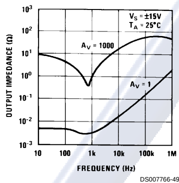
Closed Loop Output Impedance
