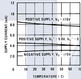
Supply Currents
