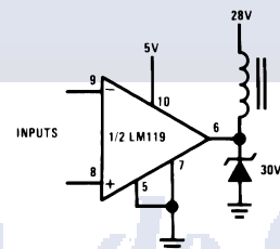
Relay Driver
