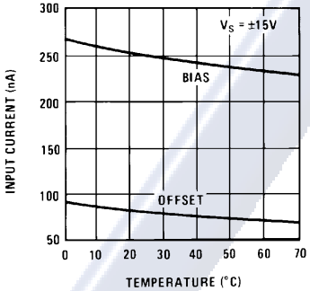
Input Currents
