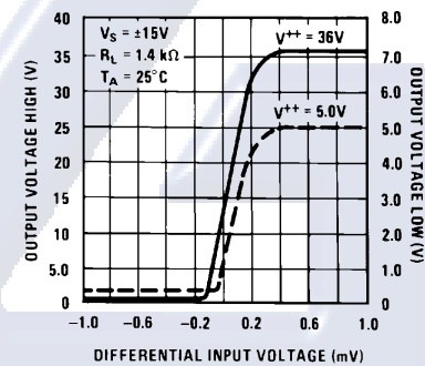
Transfer Function
