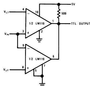
Window Detector
