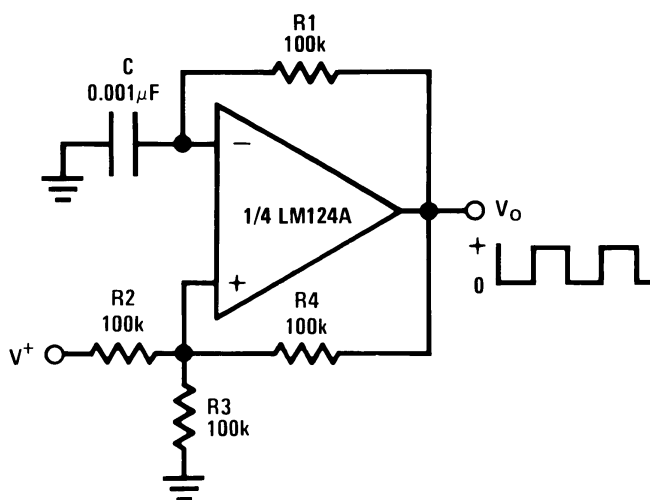
Figure 27. Squarewave Oscillator
