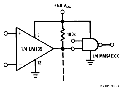
Driving CMOS
