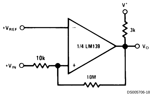
Non-Inverting Comparator with Hysteresis
