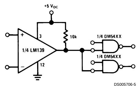
Driving TTL
