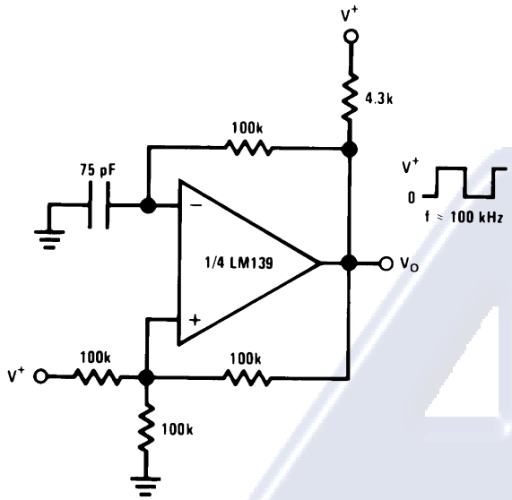
Squarewave Oscillator
