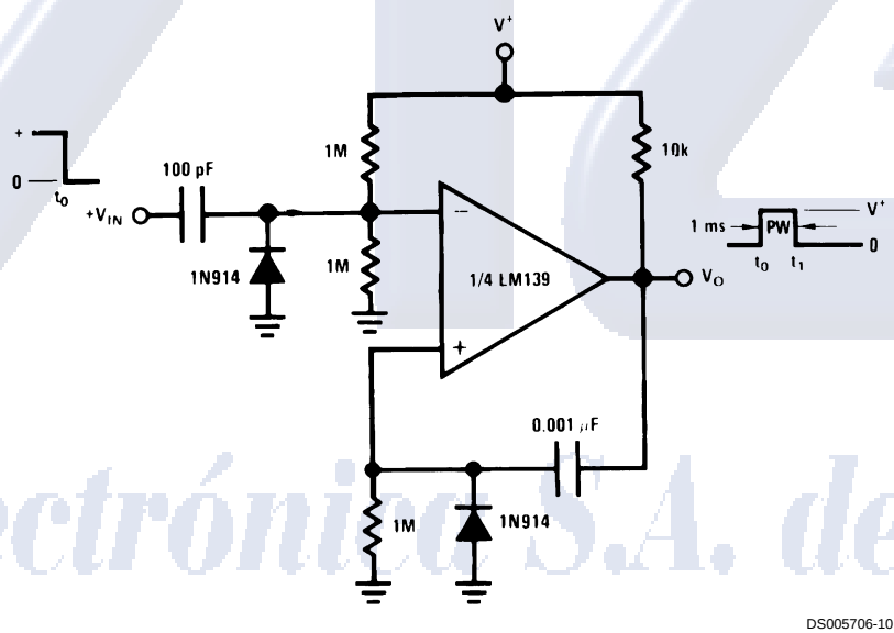
One-Shot Multivibrator
