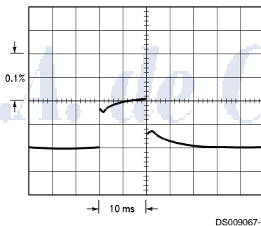
LM137, V_{OUT} = -10V V_{IN} - V_{OUT} = -40V I_L = 0A \rightarrow 0.25A \rightarrow 0A Vertical sensitivity, 5 mV/div
