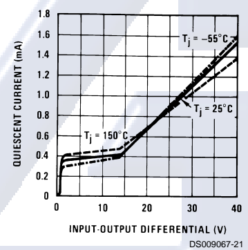
Minimum Operating Current
