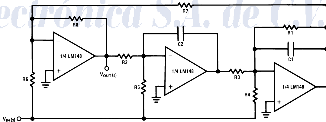
A 3 Amplifier Bi-Quad Notch Filter
