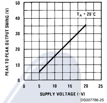
Voltage Swing
