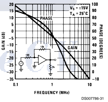
Bode Plot LM148
