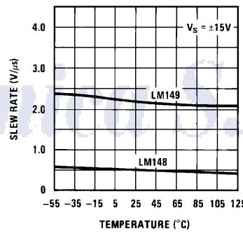
Slew Rate
