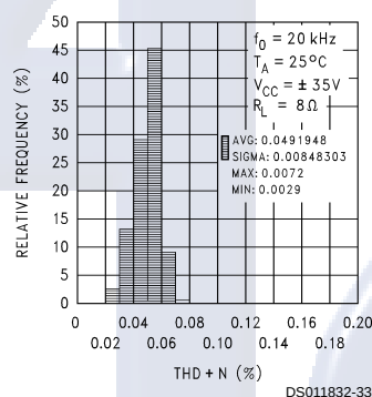
THD+N Distribution
