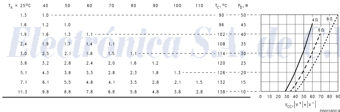
Max Heatsink Thermal Resistance (°C/W) at the Specified Ambient Temperature (°C) PDmax vs Supply Voltage
