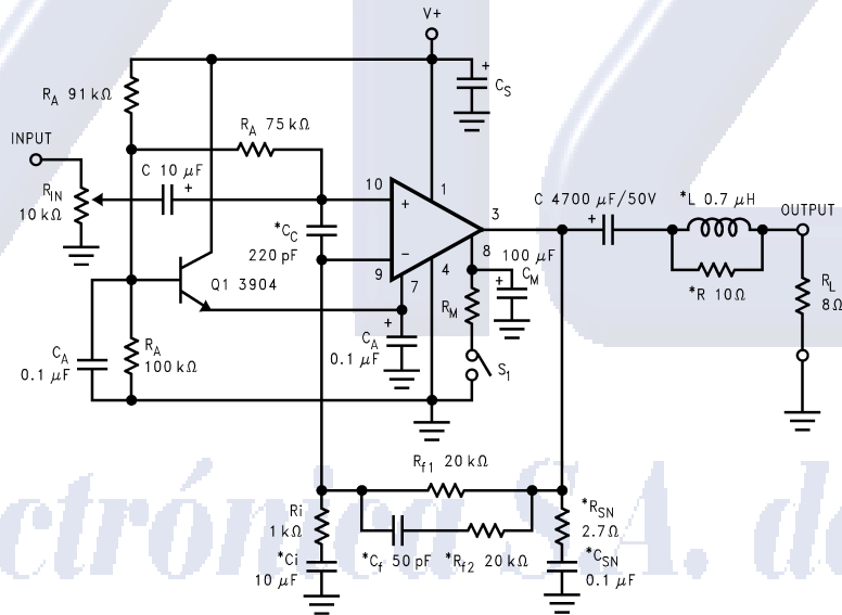
FIGURE 2. Typical Single Supply Audio Amplifier Application Circuit
