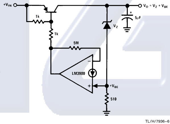
Low V_{\text{IN}} - V_{\text{OUT}} Voltage Regulator
