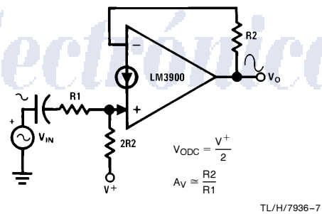
Non-Inverting Amplifier
