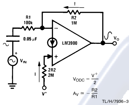
Inverting Amplifier
