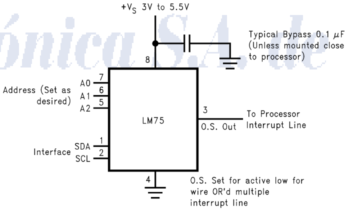
FIGURE 1. Typical Application
