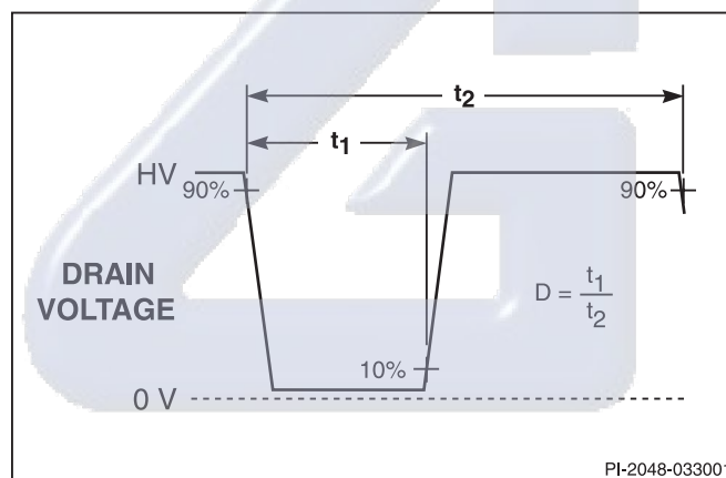
Figure 14. Duty Cycle Measurement.
