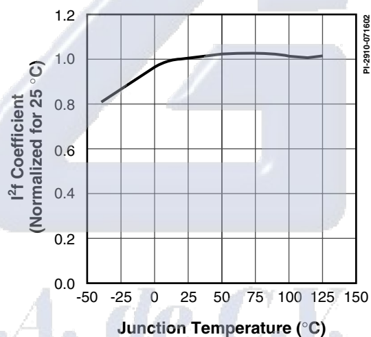
Figure 20. I^2t Coefficient vs. Temperature.
