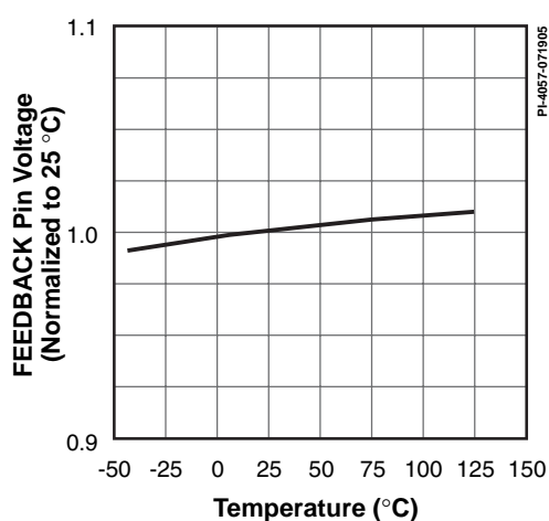
Figure 14. FEEDBACK Pin Voltage vs. Temperature.
