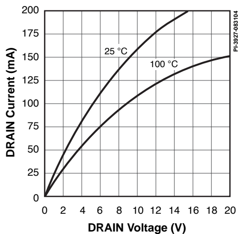
Figure 16. Output Characteristics.
