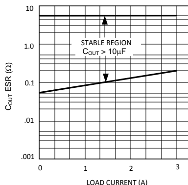
Figure 21. ESR Curve
