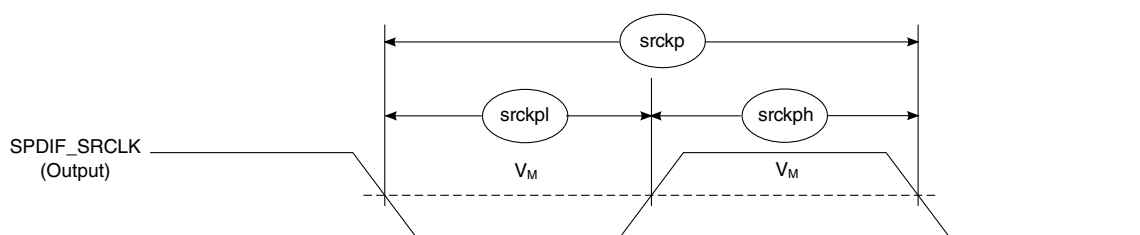
Figure 50. SPDIF_SRCLK timing
