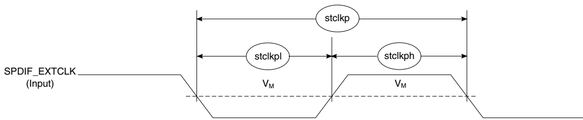
Figure 51. SPDIF_EXTCLK timing
