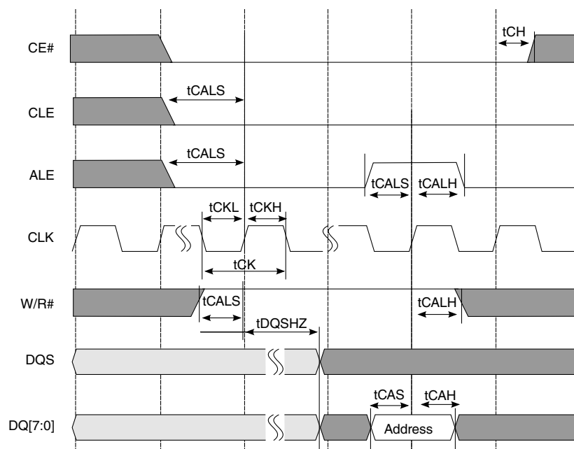
Figure 43. Address cycle
