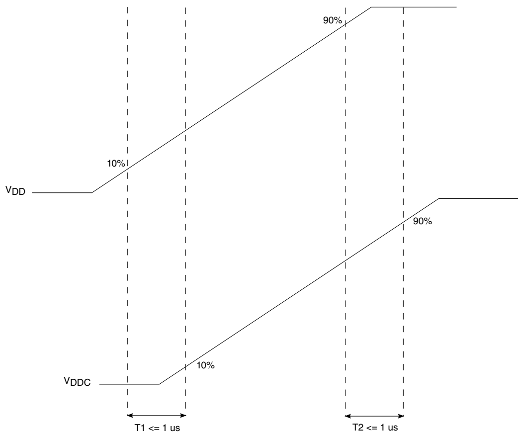
Figure 8. V_{DDC} and V_{DD} ramp-up diagram
