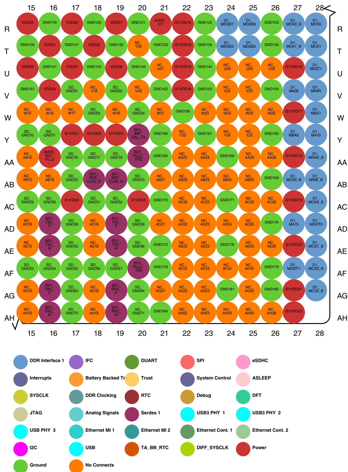
Figure 12. Detail D
