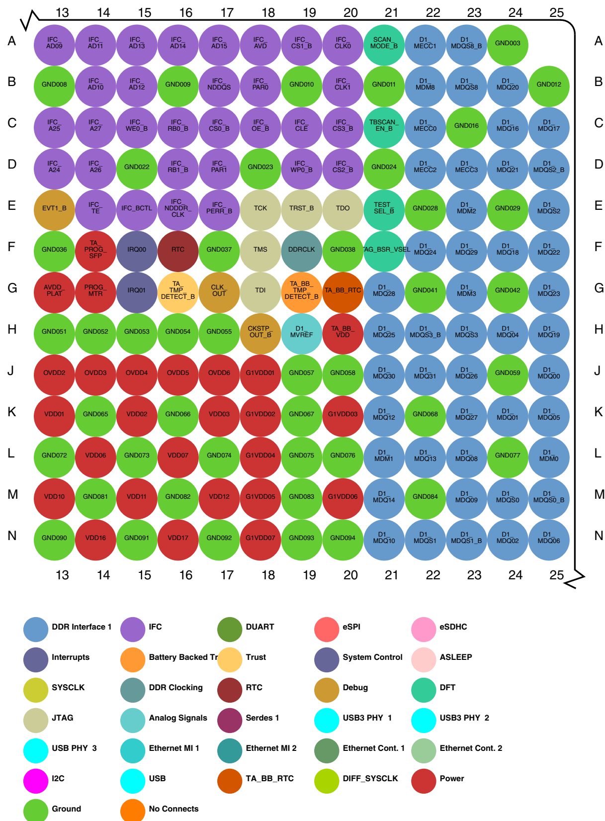
Figure 5. Detail B
