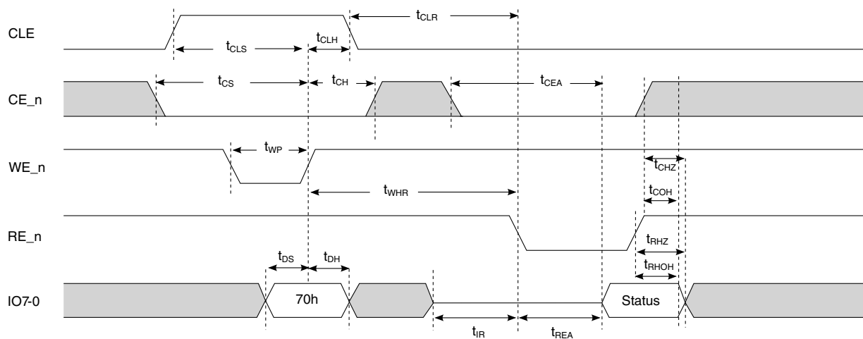
Figure 49. Read Status Timings
