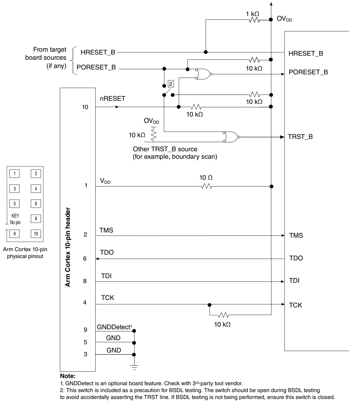
Figure 100. JTAG interface connection
