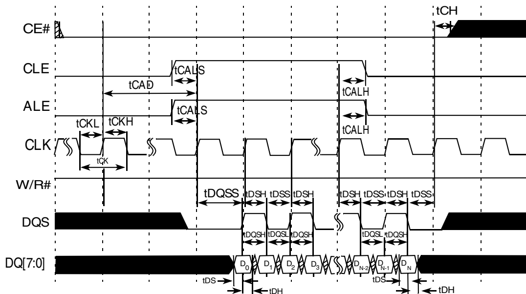
Figure 59. Write Cycle
