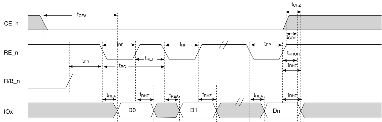
Figure 46. Data Input Cycle Timings
