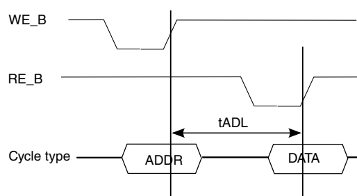
Figure 43. tADL Timing
