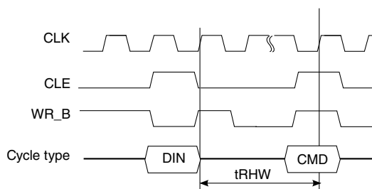
Figure 50. tRHW Timings
