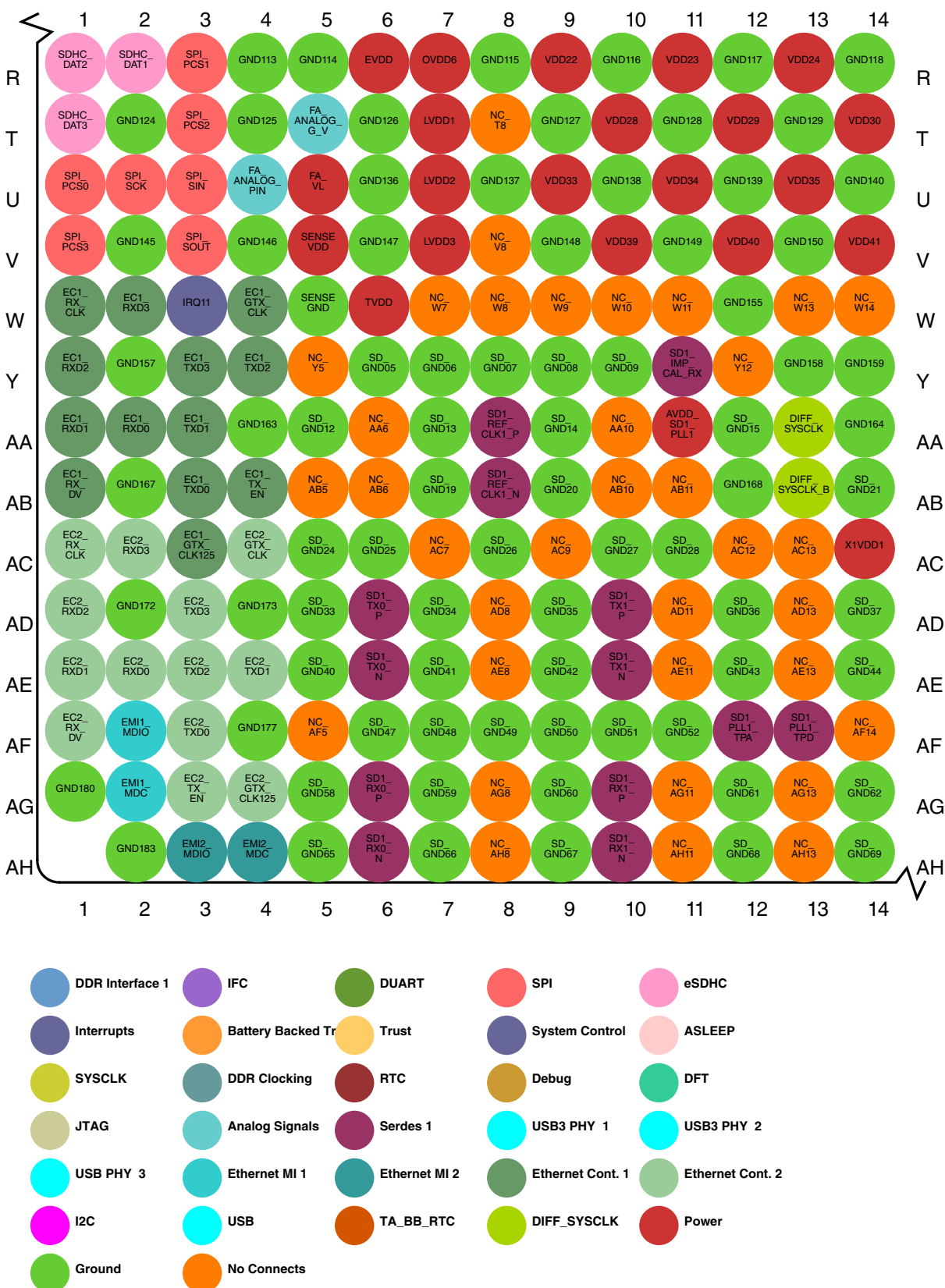
Figure 11. Detail C
