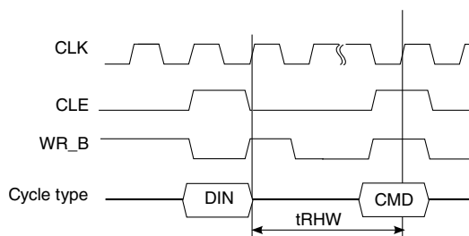
Figure 63. t_{RHW} Timings
