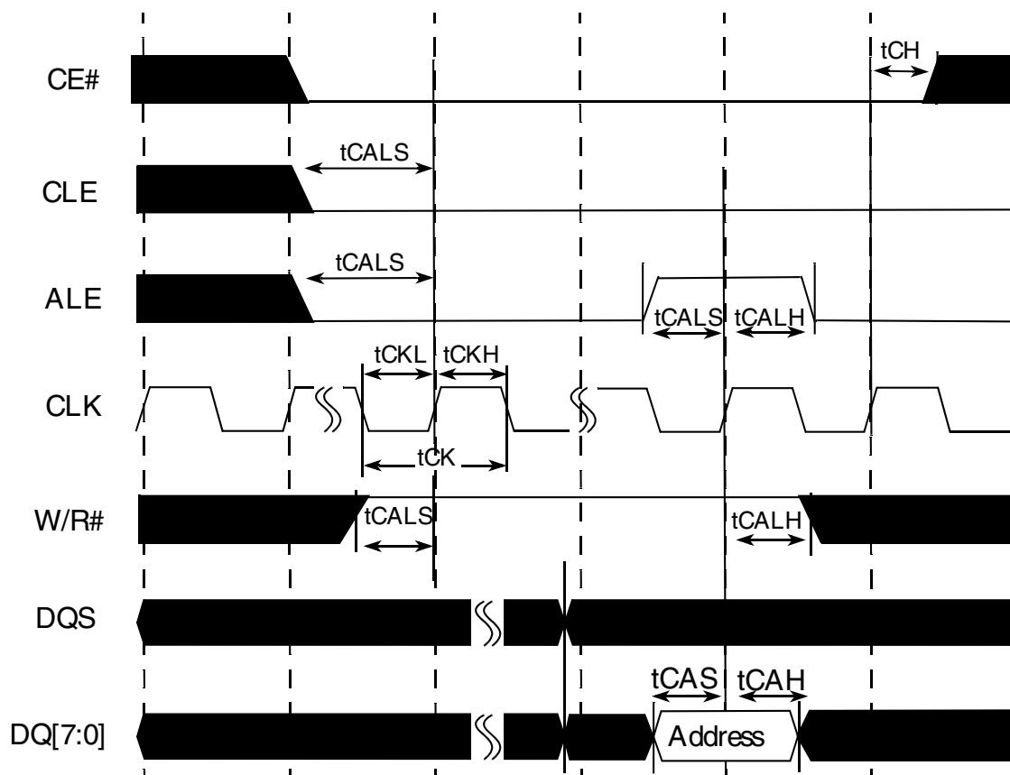
Figure 58. Address Cycle
