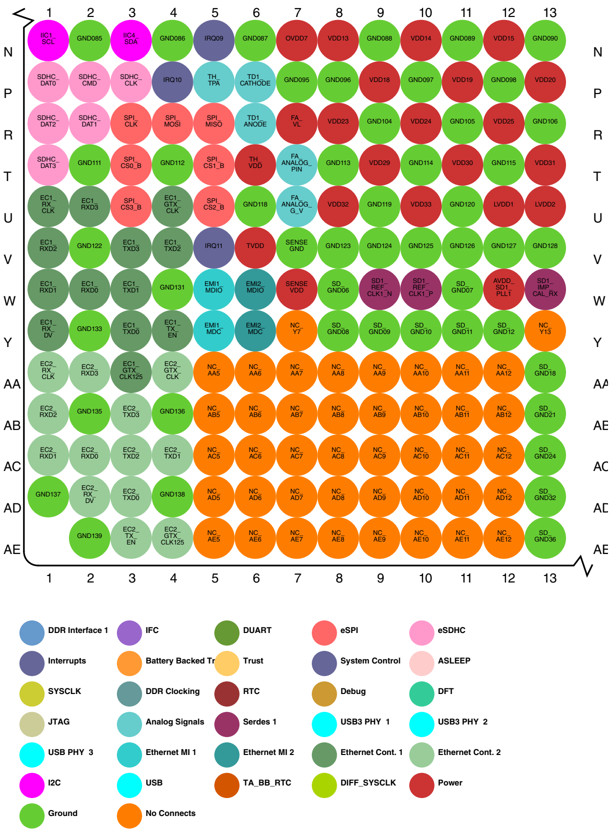
Figure 6. Detail C
