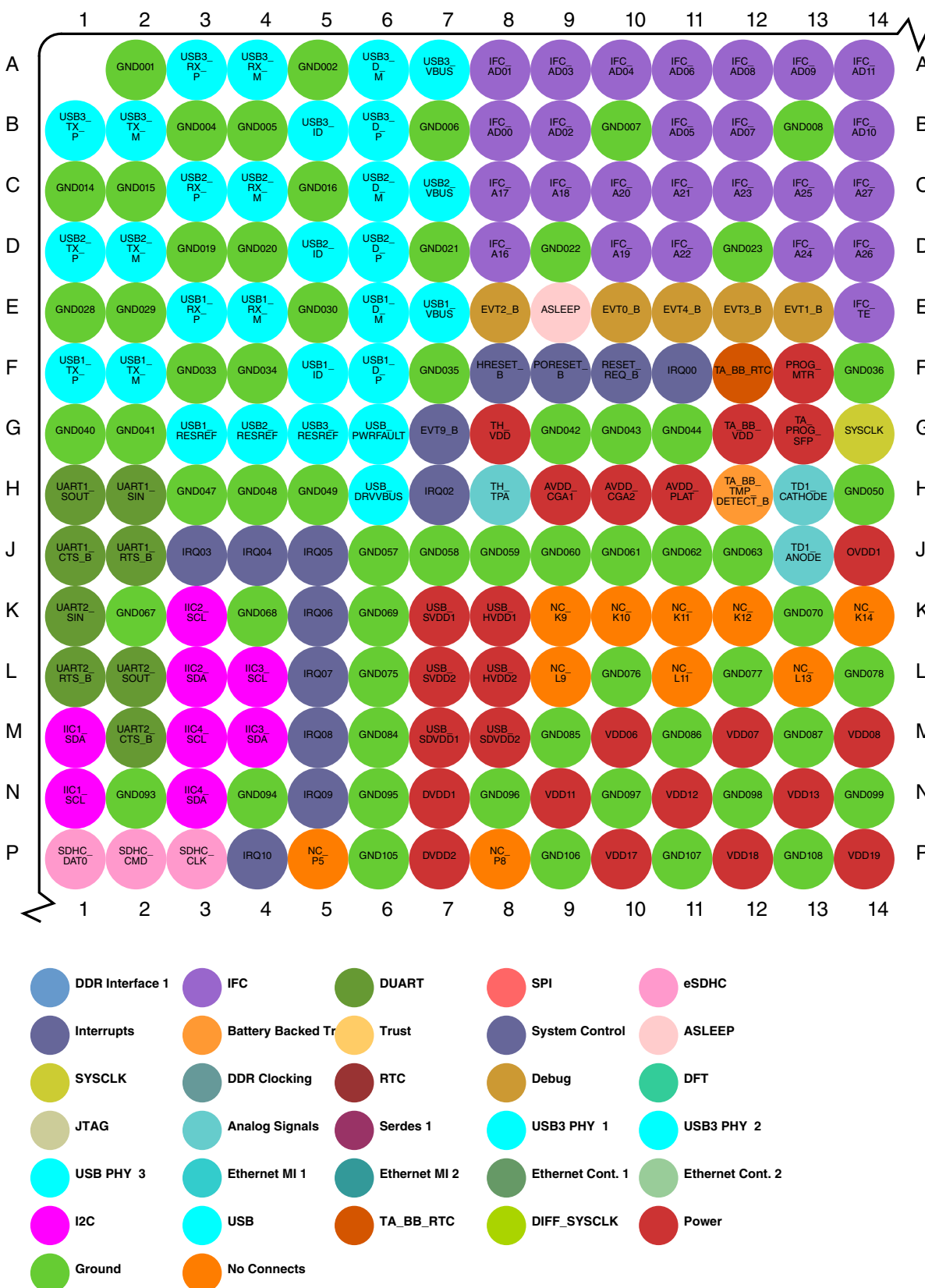
Figure 9. Detail A
