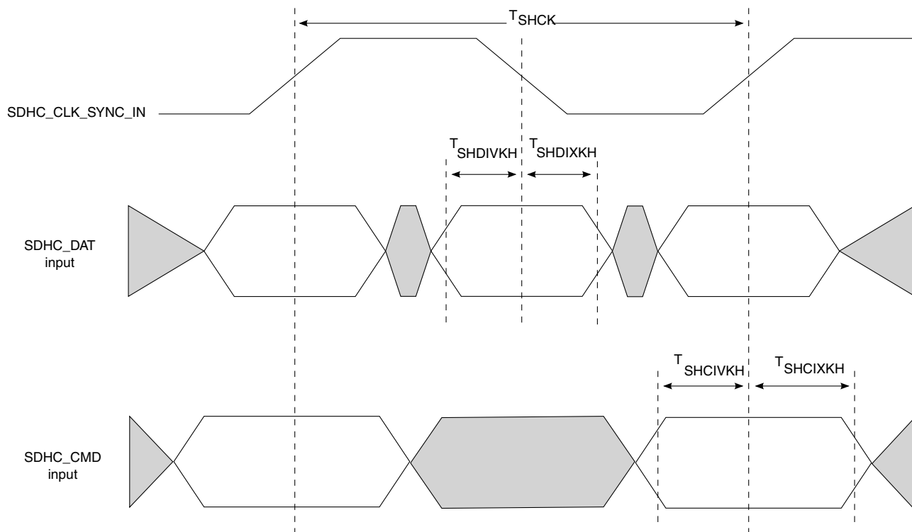
Figure 77. eSDHC DDR50/DDR mode input AC timing diagram
