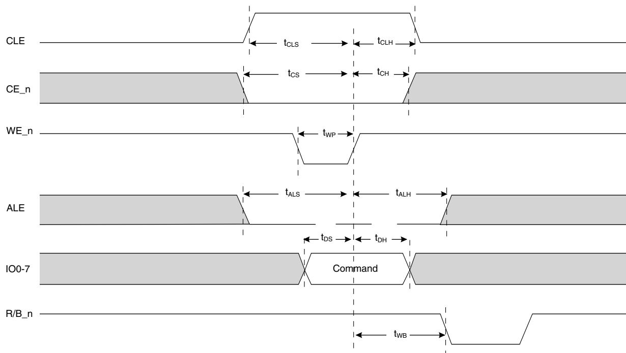
Figure 44. Command Cycle
