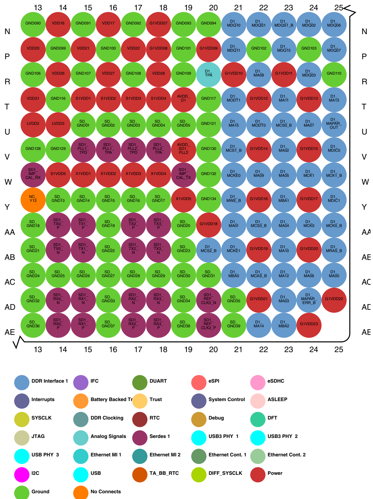
Figure 7. Detail D
