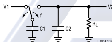
Figure 3. Switched-Capacitor Building Block
