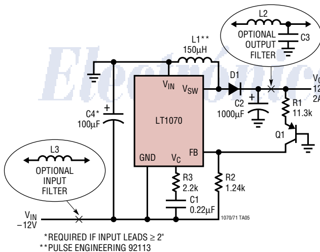
Negative to Positive Buck/Boost Converter
