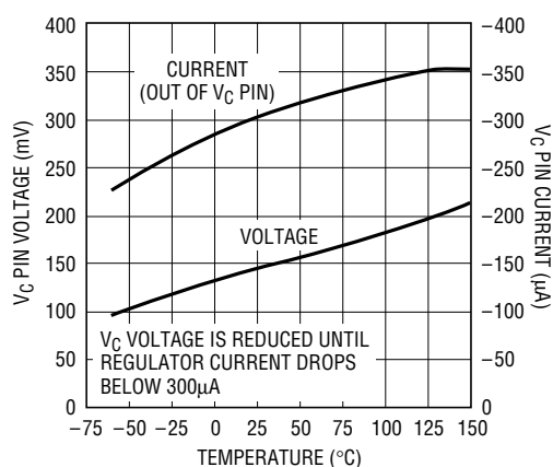
Shutdown Thresholds
