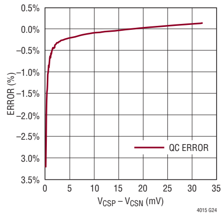
Coulomb Counter Accuracy vs V_{CSP} - V_{CSN}
